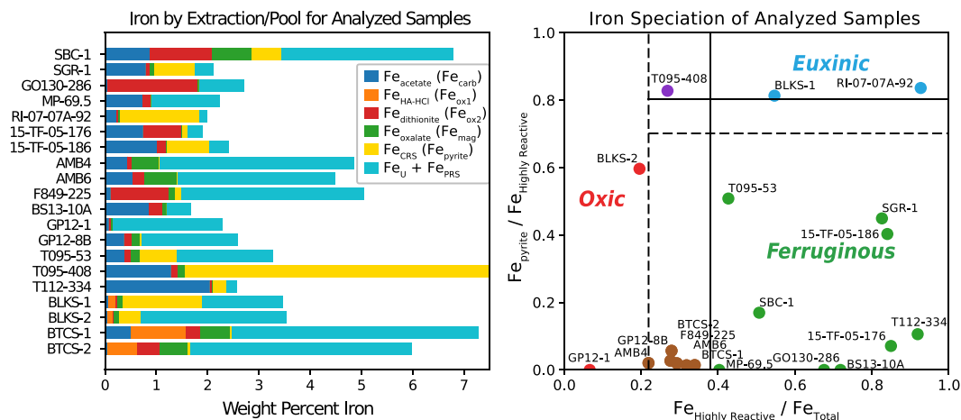
Figure 1. Iron speciation of the 20 samples shown with details of the iron extracted at each step on the left and plotted within the iron speciation proxy framework for paleoredox on the right. The pools in the bar plot are colored by the chemical extraction with the more commonly used abbreviations signaling the targeted mineralogy shown in parentheses in the legend (Poulton & Canfield, 2005). Abbreviations: carb = carbonate, HA-HCl = hydroxylamine-HCl, ox1 = easily reducible oxides, ox2 = reducible oxides, mag = magnetite, CRS = chromium reducible sulfur, U = unreactive, PRS = poorly reactive sheet silicates, Fe Highly Reactive = Fe acetate + Fe HA-HCl + Fe dithionite + Fe oxalate + Fe CRS . Note: T095-408 is off scale on the bar plot—see Tables 1 and S1 for additional information and data on all samples.
