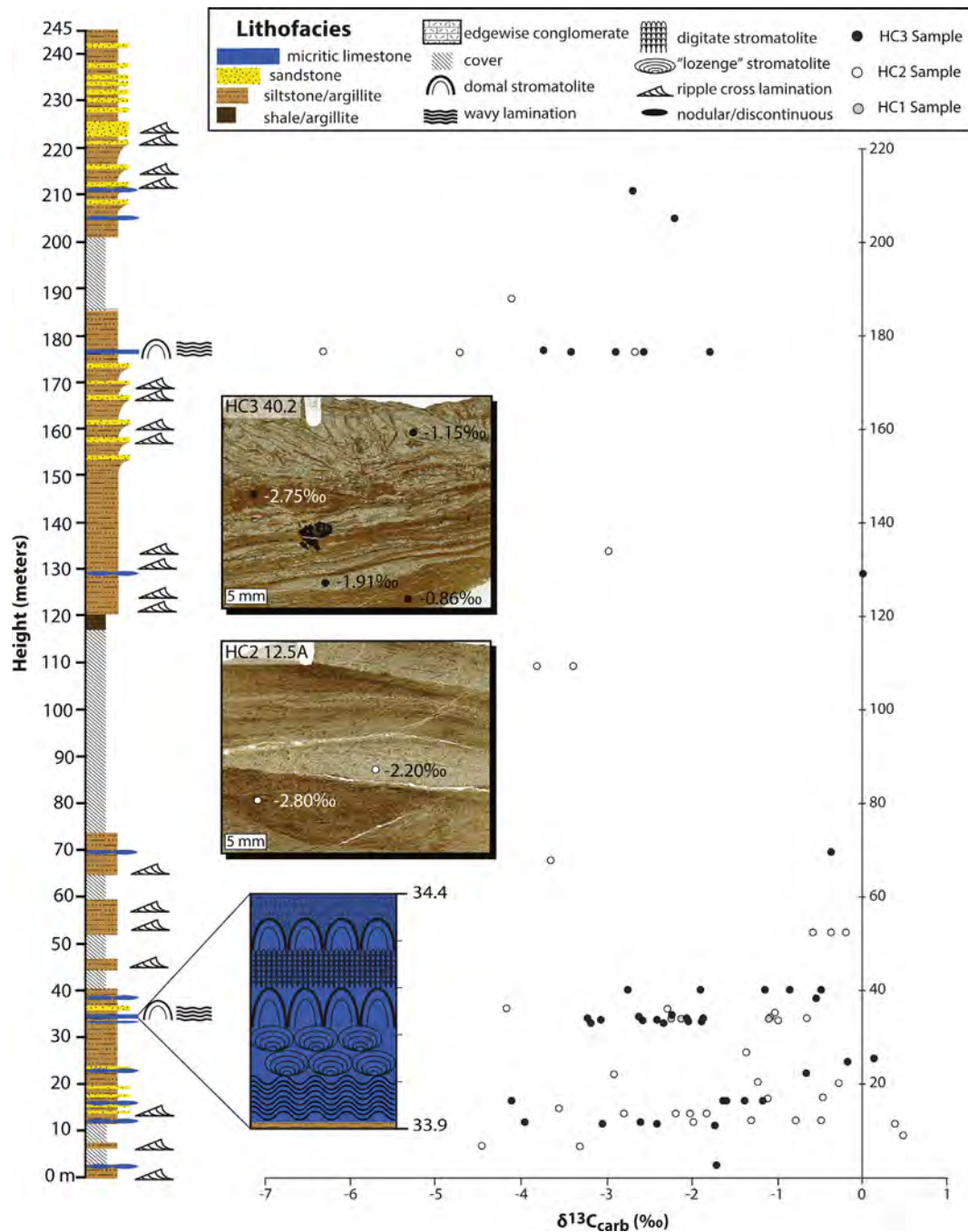
Fig. 2. Litho- and chemostratigraphy of the Kungarra Formation section at Horseshoe Creek (composite section of stratigraphic columns HC1, HC2, and HC3). The stratigraphic interval between 33.9 m and 34.4 m has been enlarged to show the succession of stromatolitic textures (interpreted to be of microbial origin). Inset images are photomicrographs (plane polarized light) of the Kungarra carbonates; sample HC2 12.5A is from 13.8 m and HC3 40.2 is from 40.2 m. Dots in inset images indicate microsampling locations and their carbon isotope values.
