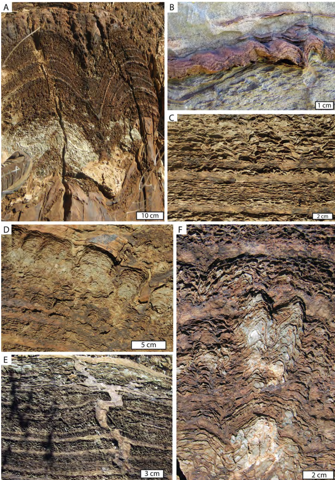
Fig. 10. Kazput stromatolites. (A) Large domal stromatolites forming over relict topography at 47 m stratigraphic height (in section K2C). (B) Thin stromatolite layer within fine-grained micritic limestones; note the eroded base on which the stromatolite accreted. (C) Alternating layers of siliciclastic lamina-rich (resistant) and carbonate-rich (recessive) layers within the larger stromatolites; note the weathering difference between units. (D) Top layers of domal stromatolites from K2C (47 m), note the alternating layers of siliciclastic lamina-rich and carbonate-rich layers. The stromatolites on the top layer formed much larger (>5 cm), more cement-rich structures than earlier layers. (E) Synsedimentary neptunian dyke through stromatolite layers, dark patches are shadows from vegetation on the outcrop. (F) Domal stromatolites growing into microdigitate stromatolites within cement-rich intervals of the large domal stromatolites in K2C.
