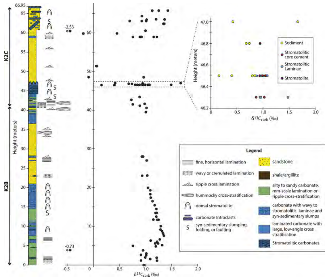
Fig. 9. Litho- and chemostratigraphy of Kazput Formation at sections K2B and K2C. Expanded section in upper right highlights geochemical results from stromatolite microsampling.
