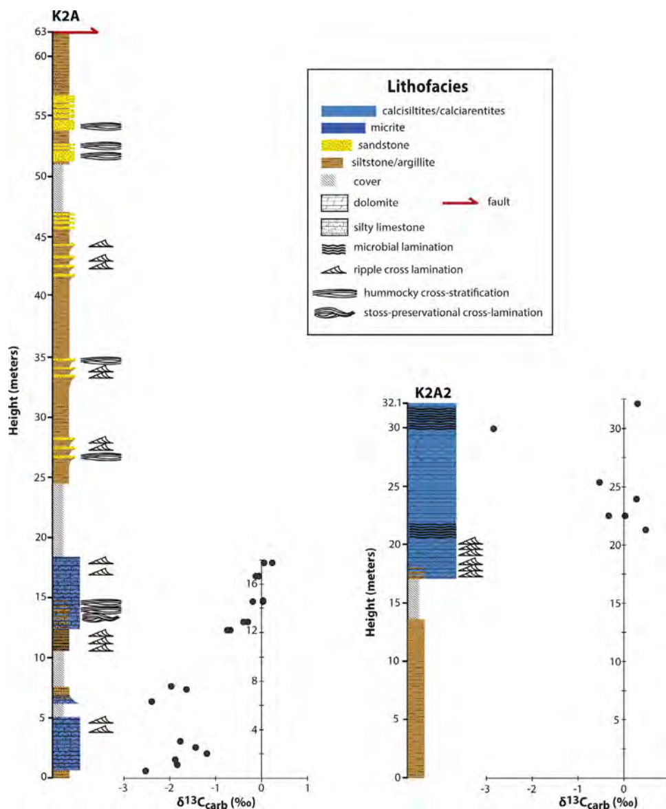
Fig. 8. Litho- and chemostratigraphy of the Kazput Formation at sections K2A and K2A2. Note that K2A2 sits stratigraphically above the K2A section.
