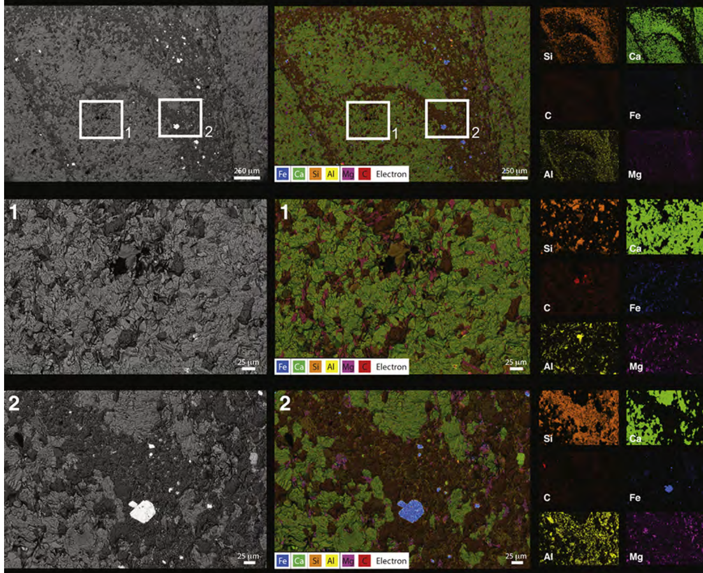
Fig. 12. Elemental map of Kazput Formation stromatolitic carbonates (sample KAZS1, 47 m height in section K2C); top row is an image of the entire sample, and the middle and bottom rows are close up views of boxes 1 and 2 respectively. Left column are SEM images, right column images are false color representations of the elemental maps, and the middle illustrations are composite images of the elemental and SEM maps. Note, unlike the Kungarra Fm. (Fig. 4), calcium (calcite) is the dominant mineral with quartz and aluminosilicates occurring with high relative abundance in stromatolitic laminae. Small iron oxide grains (blue in false color maps) occur throughout the Kazput section but are concentrated in silicate-rich laminae (orange in false color maps). There are also organic carbon inclusions throughout the section (see second row); they appear as black spots in the composite figure and are highlighted in red on the carbon (C) elemental map. (For interpretation of the references to color in this figure legend, the reader is referred to the web version of this article.)
