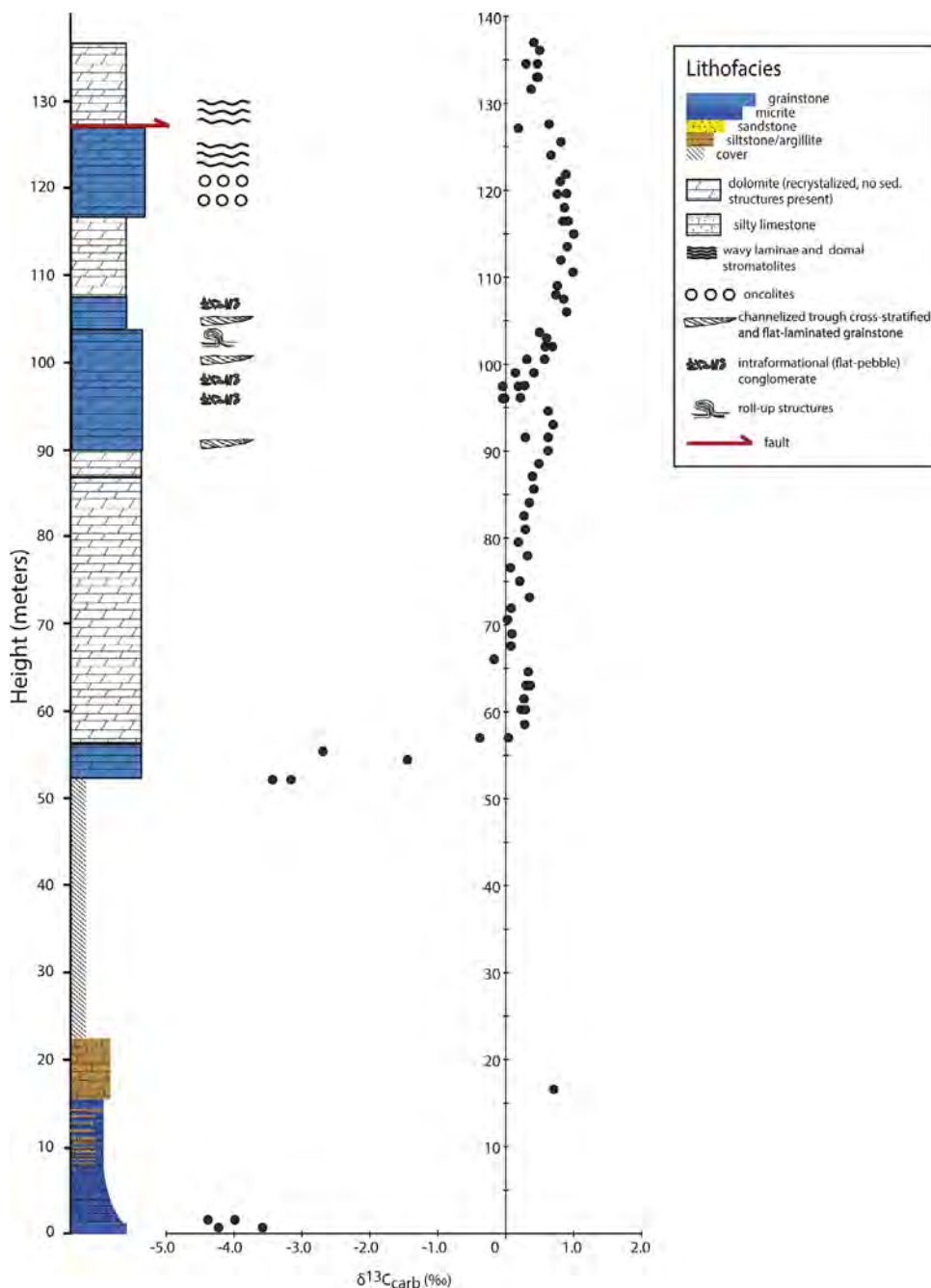
Fig. 6. Litho- and chemostratigraphy of the Kazput Formation at section K1.
