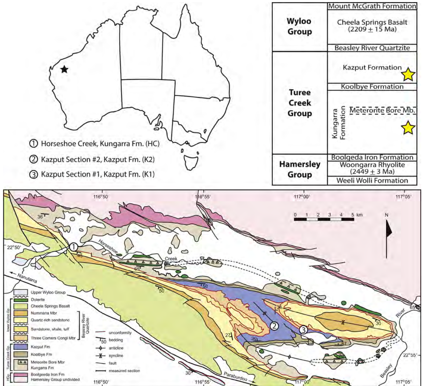
Fig. 1. Geographic, stratigraphic, and geological location of the studied sections. Upper left: location of study area in Australia (star). Upper right: stratigraphic context for the Turee Creek Group; stars indicate stratigraphic horizons of studied sections. Bottom: geological map of the Hardey Syncline from Martin et al. (2000) ; numbered circles indicate studied localities.
