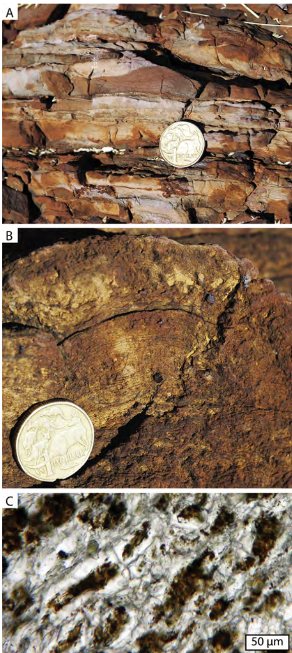
Fig. 3. Kungarra Formation carbonates at Horseshoe Creek. (A) Pinkish-white micritic limestone interbedded with reddish-brown fine-grained sandstone forming starved ripples, Australian dollar for scale (25 mm diameter). (B) Close up of stromatolites from roughly 34.2 m in stratigraphic height, Australian dollar for scale. (C) Petrographic view of the domal stromatolite layer (sample HC3 34.3, 34.3 m in stratigraphic height), showing overgrowths of calcite on micritic carbonates stained by iron oxides (note scale bar). (For interpretation of the references to color in this figure legend, the reader is referred to the web version of this article.)
