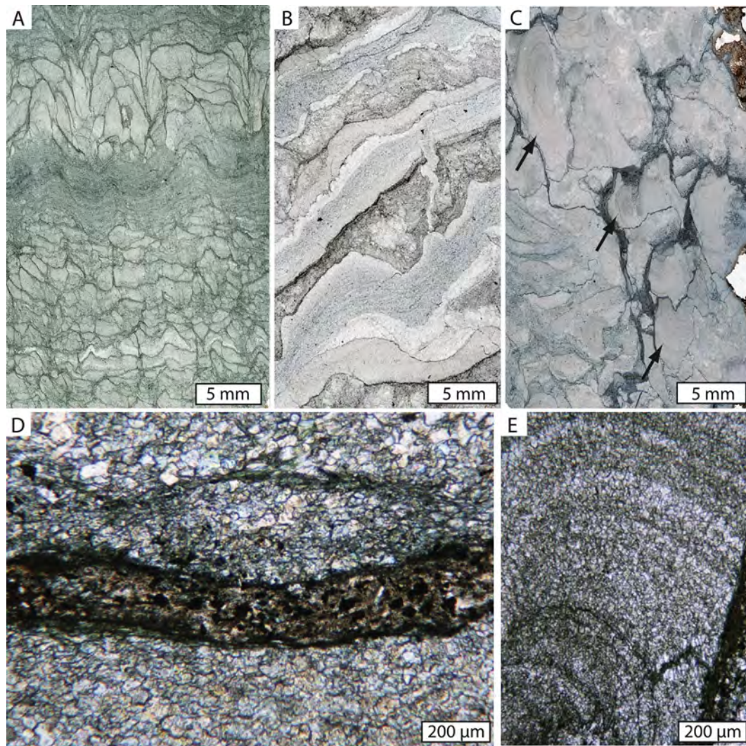
Fig. 11. Petrographic textures of Kazput stromatolites (all plane polarized light). (A) Alternating siliciclastic lamina-rich and discontinuous carbonate-rich layers of large domal stromatolites from section K2C (47 m, sample K2C 5.5B2); (B) unusually continuous carbonate-rich layers in section K2C (65.7 m, sample K2C 31.8 m); (C) microstructure of a transported and rolled up stromatolite, showing the local preservation of fine banding in lenticular carbonate precipitates highlighted by arrows (63.4 m, sample K2C 28.6); (D) detail of a siliciclastic-rich lamina in a small stromatolite containing quartz, pyrite, and clay minerals, with carbonate-rich areas above and below (sample K2C 28.5); (E) close up of (C) highlighting the faint banding within the carbonate fabric of the deformed stromatolite (63.4 m sample K2C 28.6).
