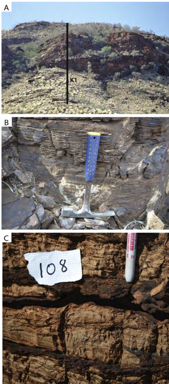
Fig. 5. Lithologies of the Kazput Formation in Hardey Syncline section K1. (A) Overview of stratigraphy, section K1 begins in the thin-bedded limestones in the foreground, the base of the cliff is at 53 m elevation in the stratigraphic column (Fig. 6), and the measured section continues up the gully on the left. (B) Close-up of thin-bedded limestones at the base of the K1 section, hammer for scale. (C) Cross-stratified grainstones with abundant bed-parallel silicification at meter 108 in the K1 section, Sharpie tip for scale.
