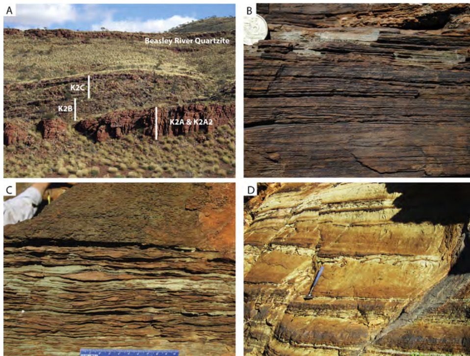
Fig. 7. Lithologies of the Kazput Formation in Hardey Syncline section K2. (A) Overview of stratigraphy, showing where individual subsections were measured. (B) Fine grained, parallel-laminated facies in section K2A, Australian dollar for scale (25 mm diameter). (C) Section K2B; silty to (fine) sandy carbonates with small-scale ripples in the lower half of the photo and mm-scale laminations in the upper half. Blue ruler at the bottom of the photo is 10.5 cm long. (D) Interbedded sandy carbonates and fine-grained carbonates with wavy to stromatolitic laminae (section K2B); rock hammer for scale.
