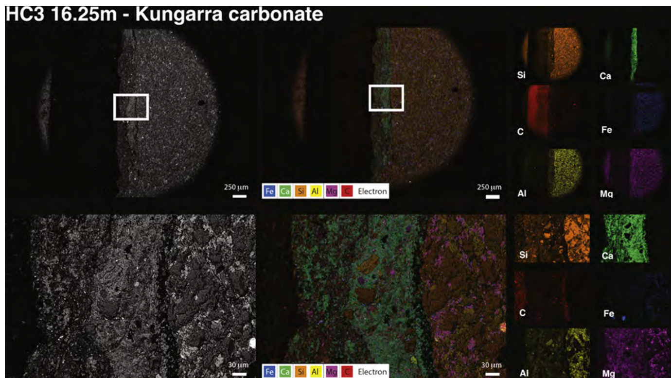
Fig. 4. Elemental map of Kungarra Formation limestone (sample HC3 16.25 from 16.25 m in stratigraphic height); top images are the entire sample, and the bottom images are close up views of the boxed area. On the left are SEM images, on the right are false color representations of the elemental maps, and the middle images are a composite image of the SEM images and elemental maps. Note that the calcium (calcite) only manifests in rare lenses with abundant detrital minerals, suggesting that it is not primary carbonate but rather diagenetic. (For interpretation of the references to color in the text, the reader is referred to the web version of this article.)
